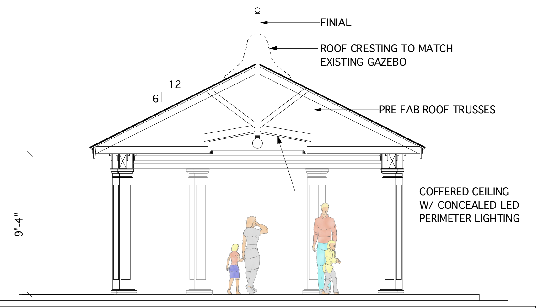
SECTION
