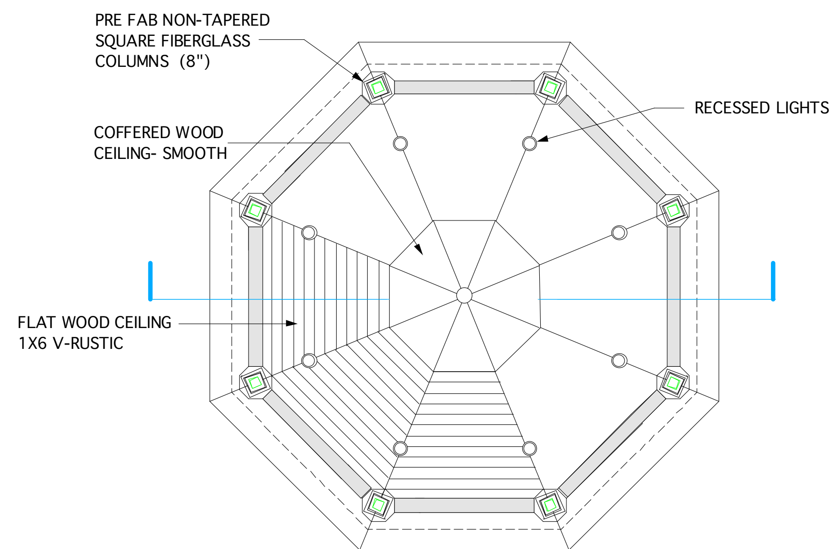
REFLECTED CEILING
