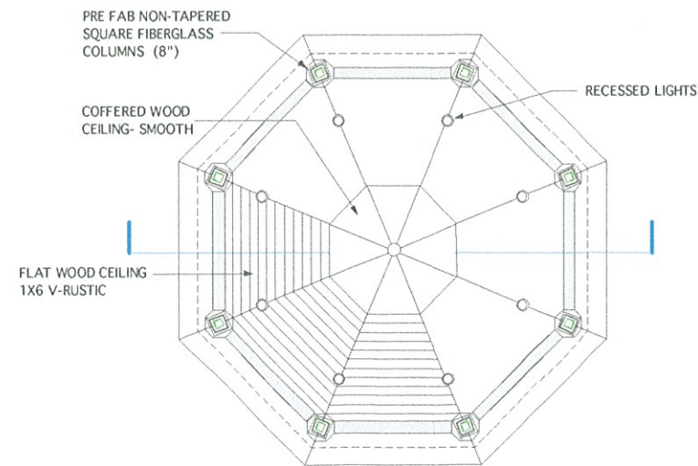
REFLECTED CEILING
