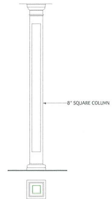
COLUMN PROFILE
