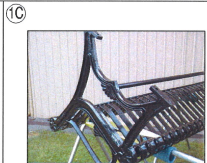
ATTACH CAST SUPPORT TO SEAT ASSEMBLY. IF HOLES IN CASTING DO NOT ALIGN WITH THE SEAT ASSEMBLY, ADJUST BY USING THE RATCHET STRAP.
